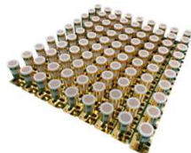
Quad Rridged Conical Horn Antenna(28GHz)
