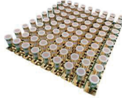
Quad Ridged Conical Horn (28GHz)
